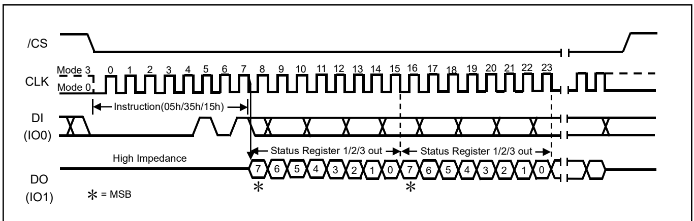
Figure4. Read Status Register Sequence Diagram
